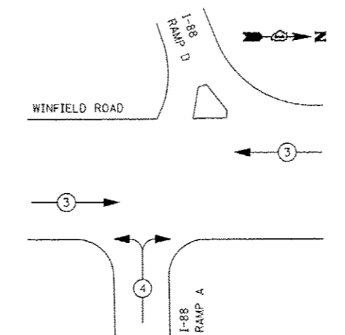
EMERGENCY VEHICLE PREEMPTION SEQUENCE ALL STAGES
