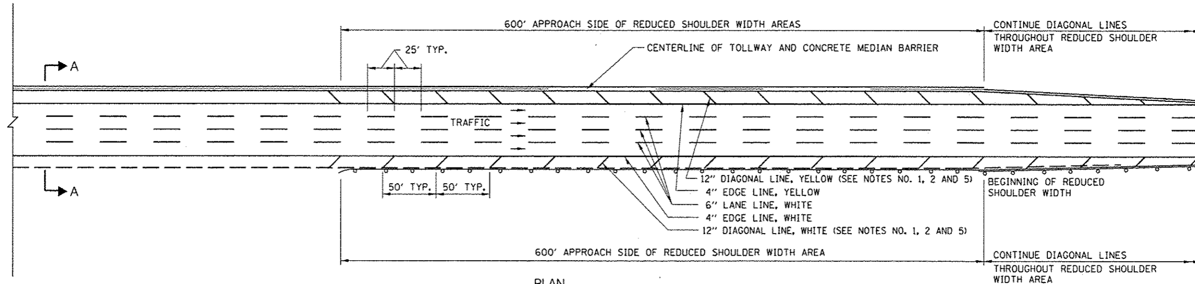
PLAN
