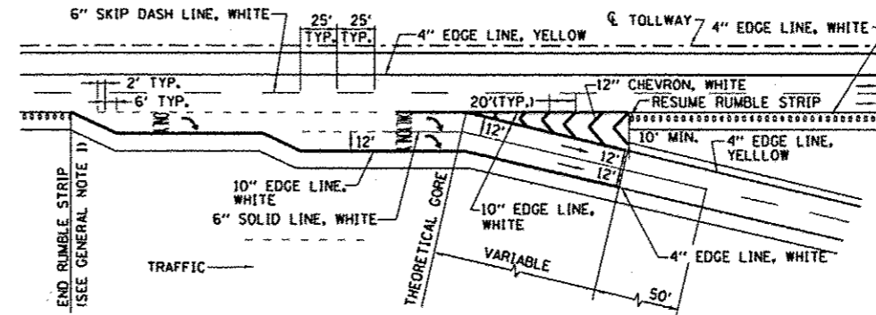
EXIT - TWO LANE PARALLEL RAMP
