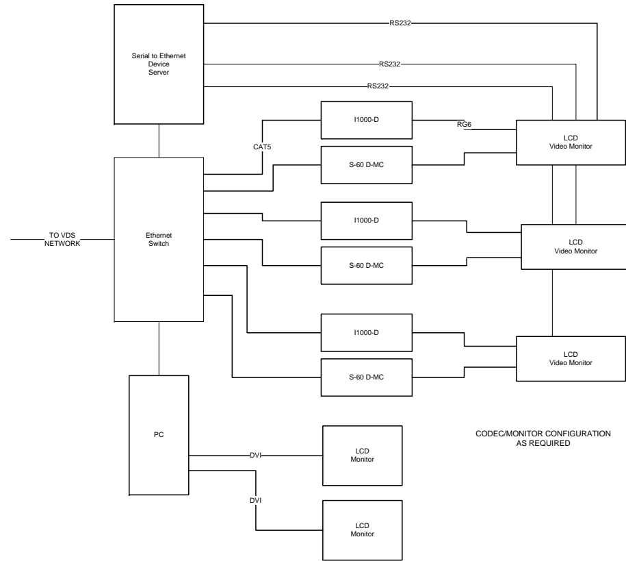
VIDEO DISTRIBUTION SYSTEM WORKSTATION TYPE A
