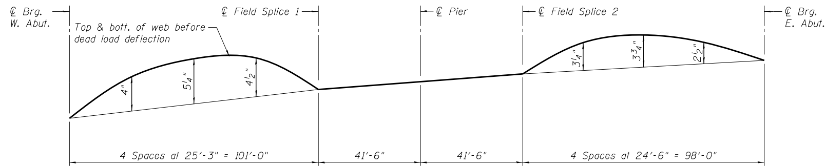
CAMBER DIAGRAM GIRDERS 1 & 2
