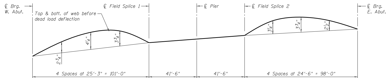
CAMBER DIAGRAM GIRDERS 3 THRU 6
