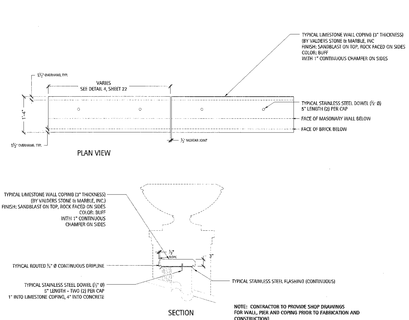
2 Typical Limestone Coping Detail Scale: 1" = 1'
