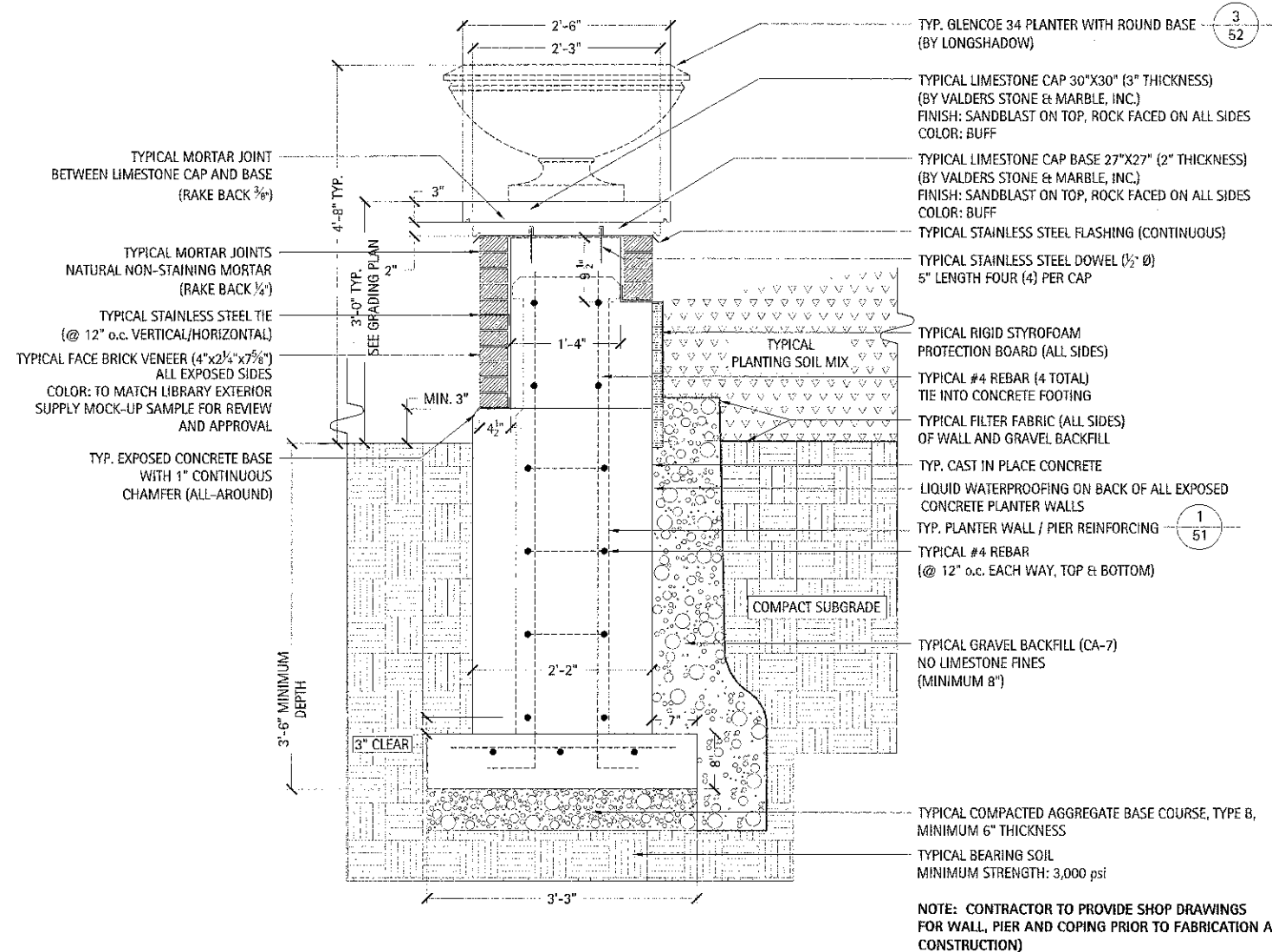
1 Typical Brick Pier Detail Scale: 1" = 1'-0"
