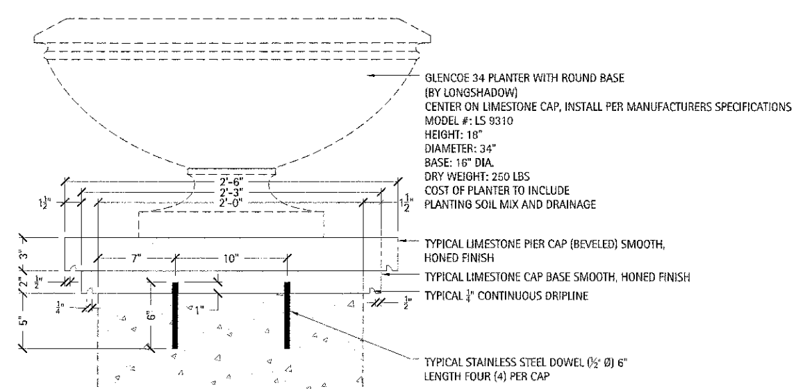
3 Typical Pier Cap Detail Scale: 1/2" = 1'
