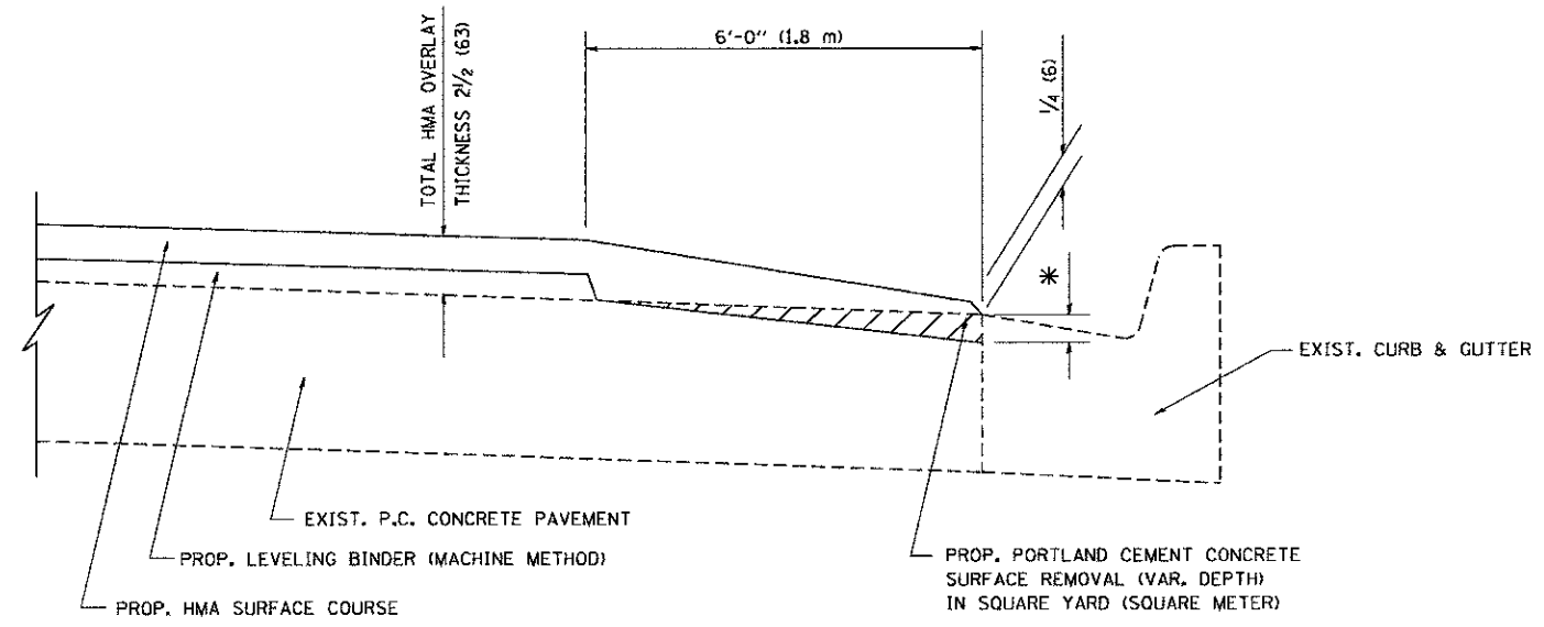
HMA TAPER AT EDGE OF P.C.C PAVEMENT
