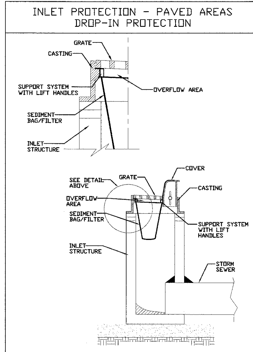
INLET FILTER
