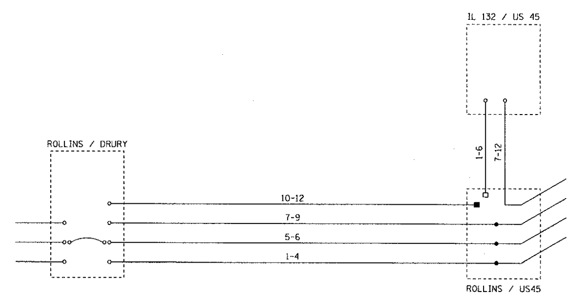
PERMANENT FIBER SPLICING DIAGRAM
