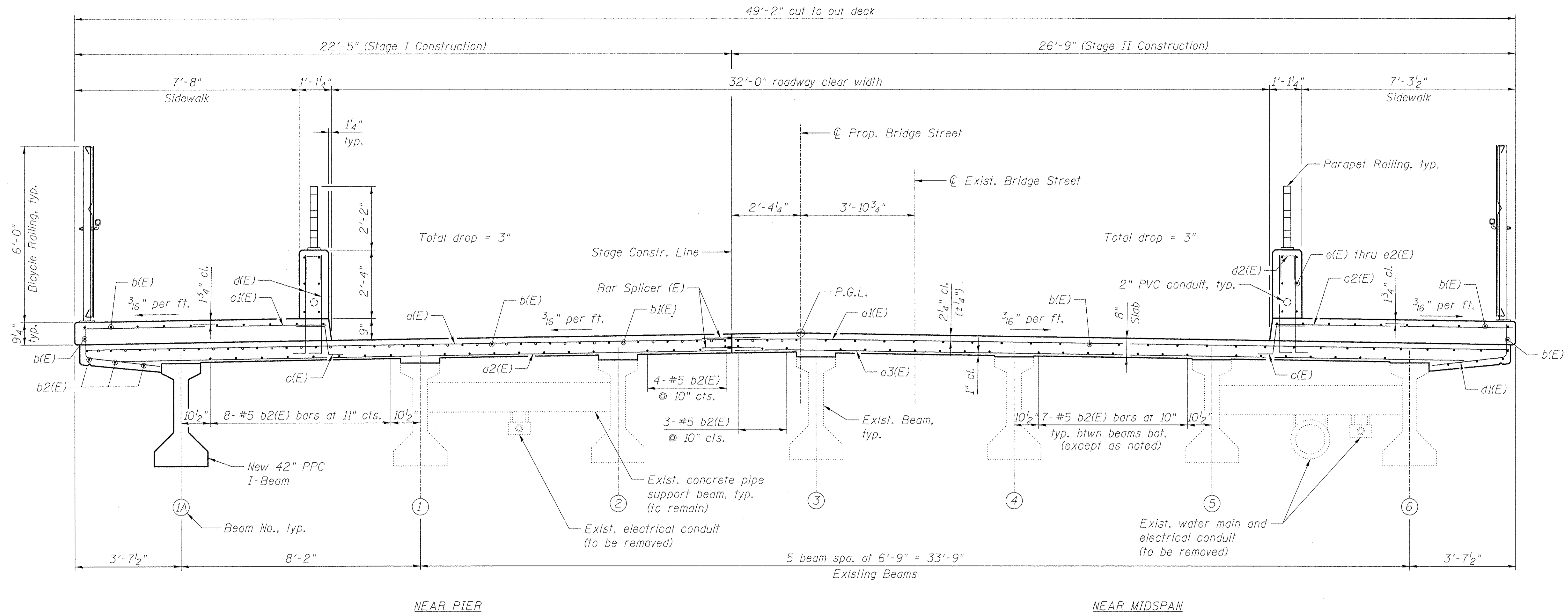
CROSS SECTION (Looking Upstation)
