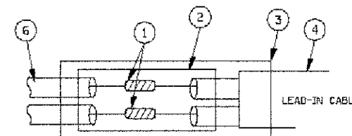
PRE-FORMED LOOP
