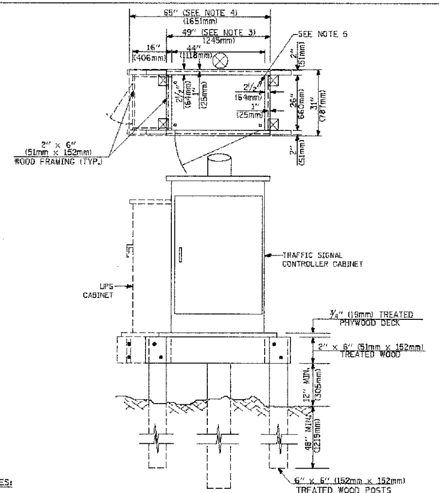
TEMPORARY SIGNAL CONTROLLER WOOD SUPPORT PLATFORM
