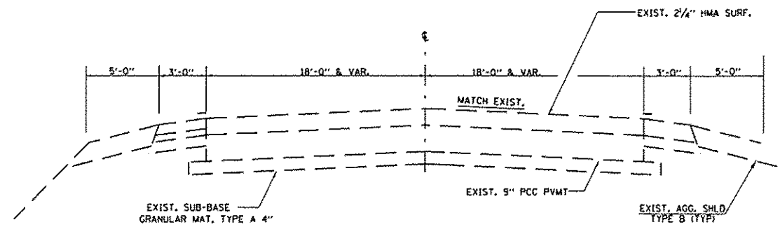
TYPICAL SECTION 6
