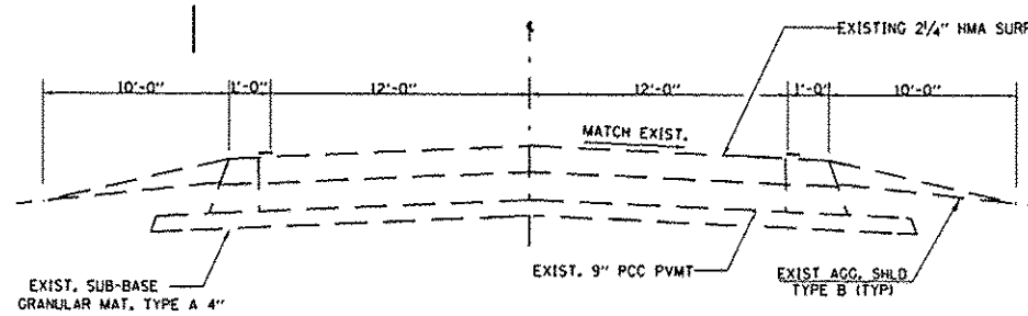
TYPICAL SECTION 7
