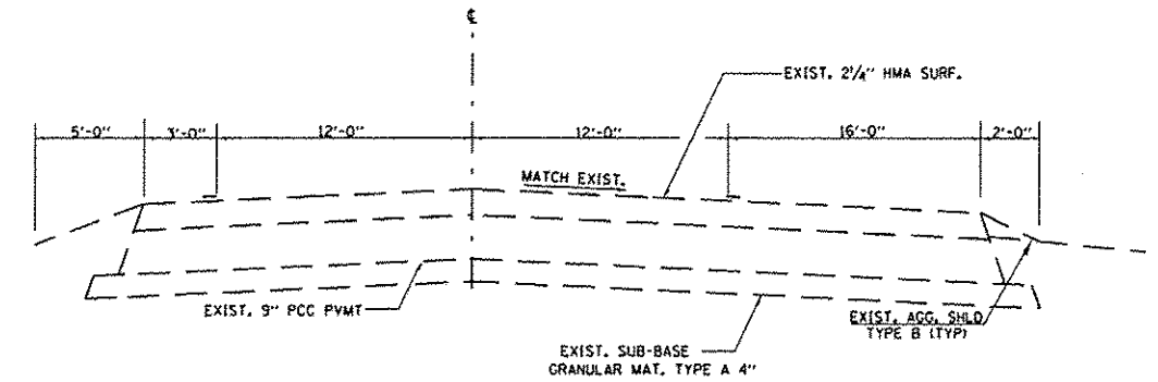
TYPICAL SECTION 5
