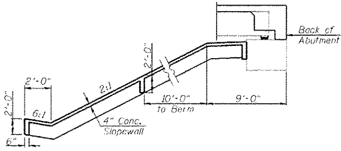
SECTION THRU SLOPEWALL
