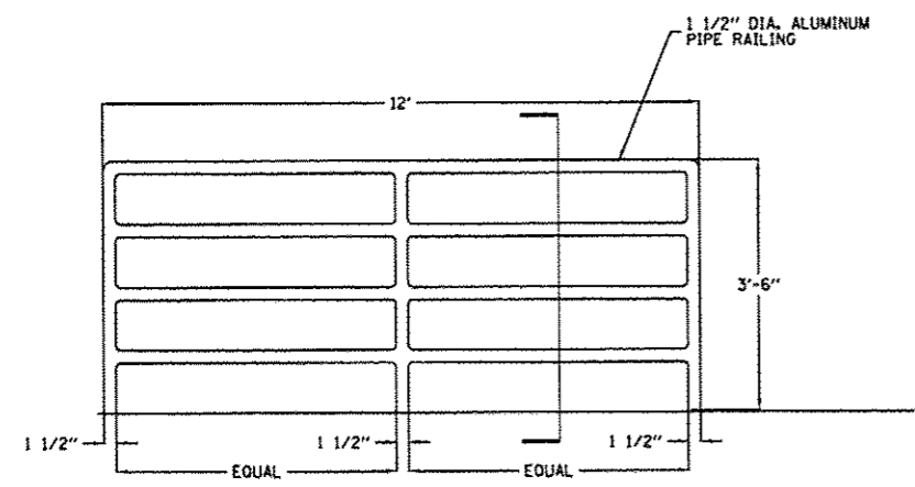
TYPICAL HANDRAIL DETAIL NO SCALE
