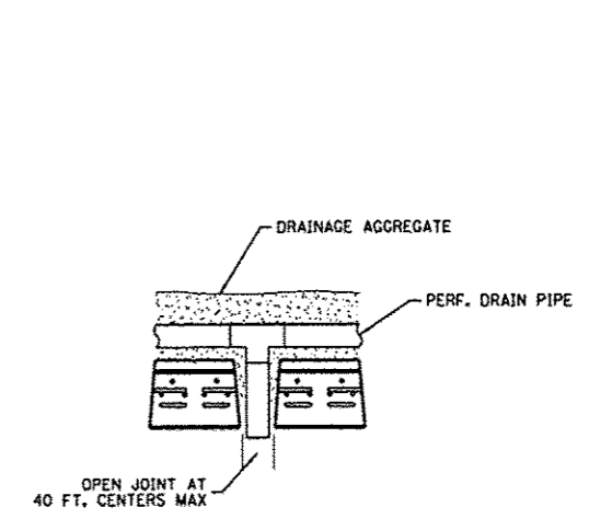
TYPICAL DETAIL NO SCALE
