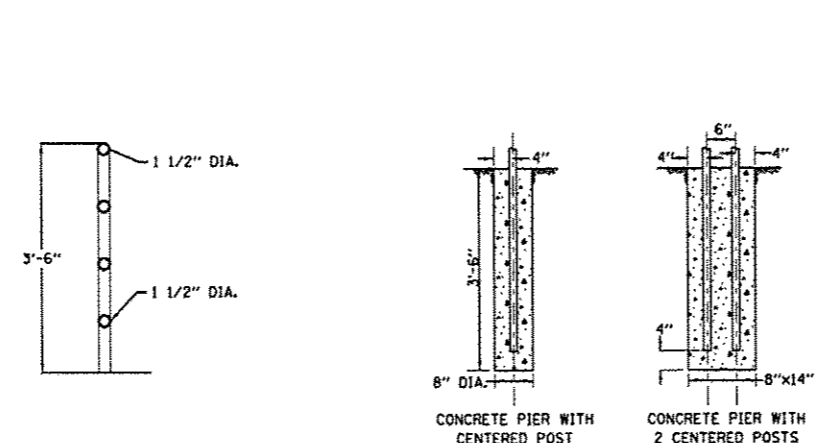
TYPICAL CONCRETE PIER DETAIL NO SCALE
