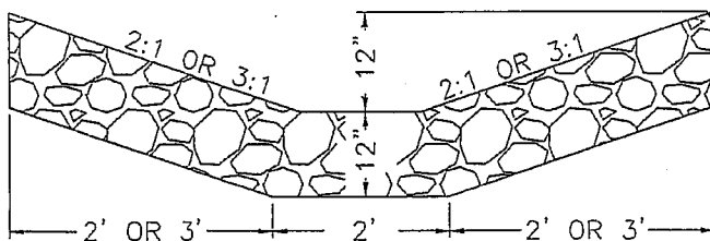
DETAIL OF AGGREGATE DITCH (SPECIAL)
