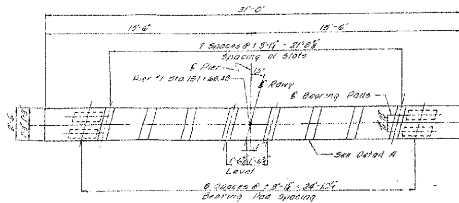
TOP PLAN
