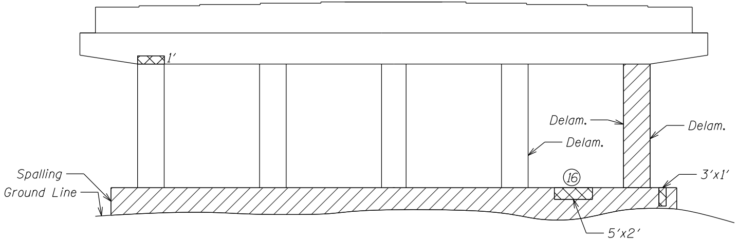
Pier 8 (Looking South)
