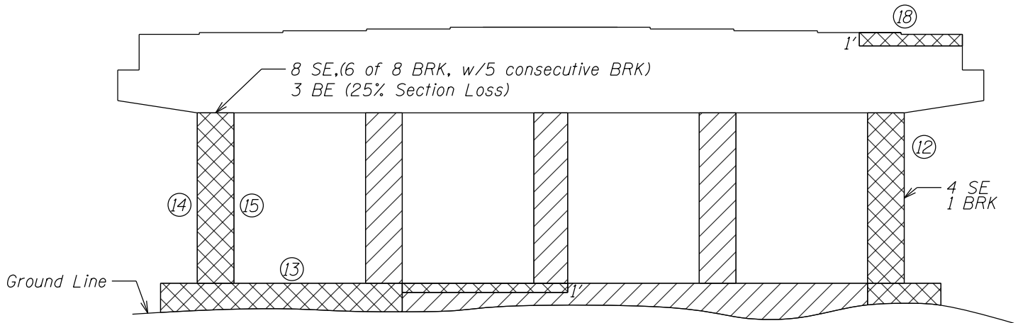
Pier 8 (Looking North)
