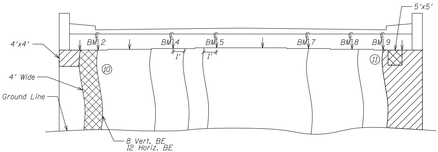
North Abutment (Looking North) All cracks from hairline to 1/16"
