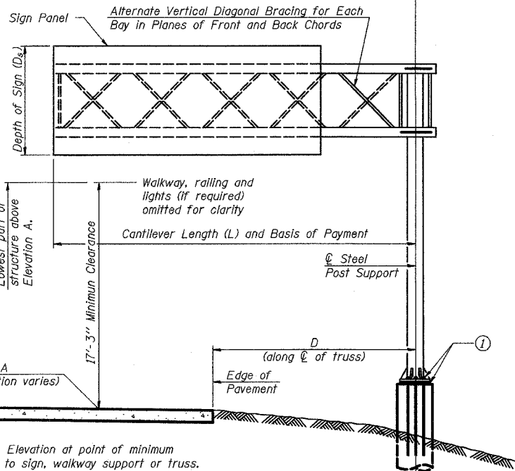
TYPICAL ELEVATION Looking in Direction of Traffic
