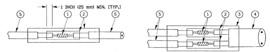
DETAIL "A" LOOP-TO-LOOP SPLICE
