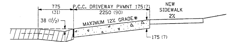
ASCENDING APPROACH
