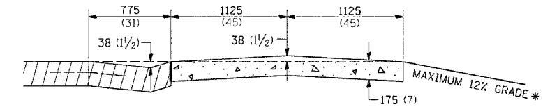
DESCENDING APPROACH
