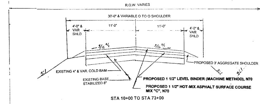
PROPOSED TYPICAL SECTIONS
