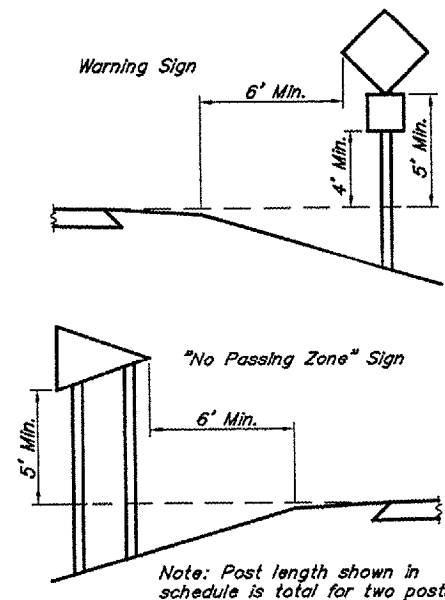
SIGN SCHEDULE & MOUNTING DETAIL
