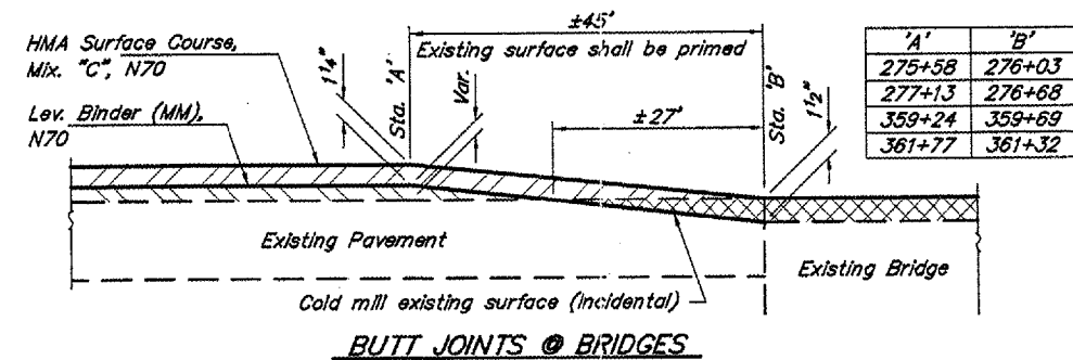
BUTT JOINTS @ BRIDGES
