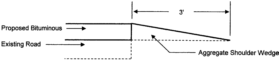
DETAIL FOR AGGREGATE SHOULDER WEDGE
