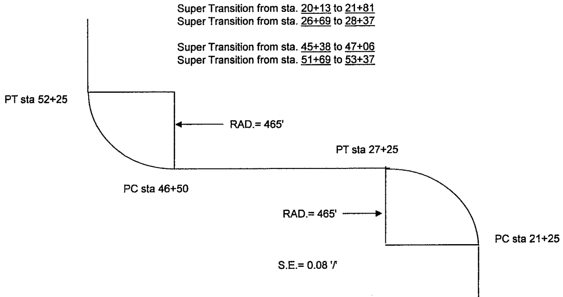
DETAIL OF SUPERELEVATION FOR CURVES 40 MPH DESIGN
