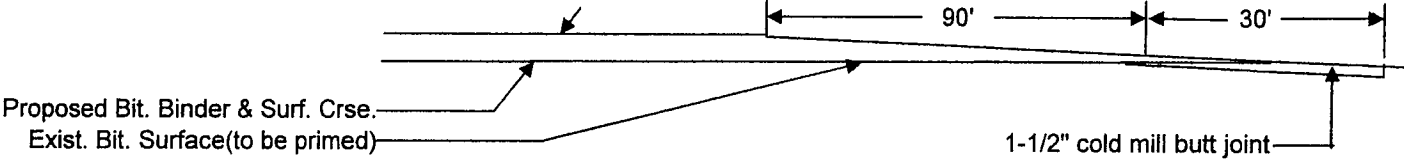
DETAIL OF BEGINNING AND ENDING TAPERS
