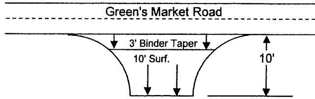
DETAIL OF PRIVATE ENTRANCE
