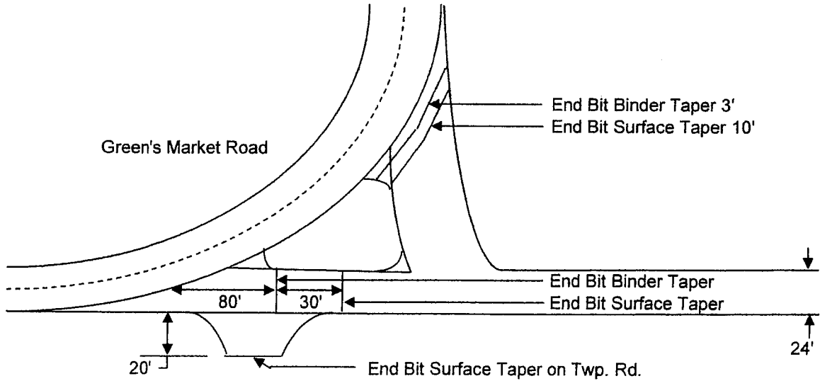
DETAIL OF SIDEROAD
