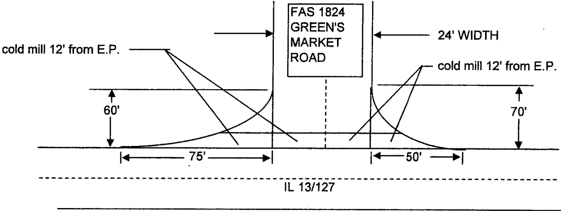
DETAIL OF INTERSECTION
