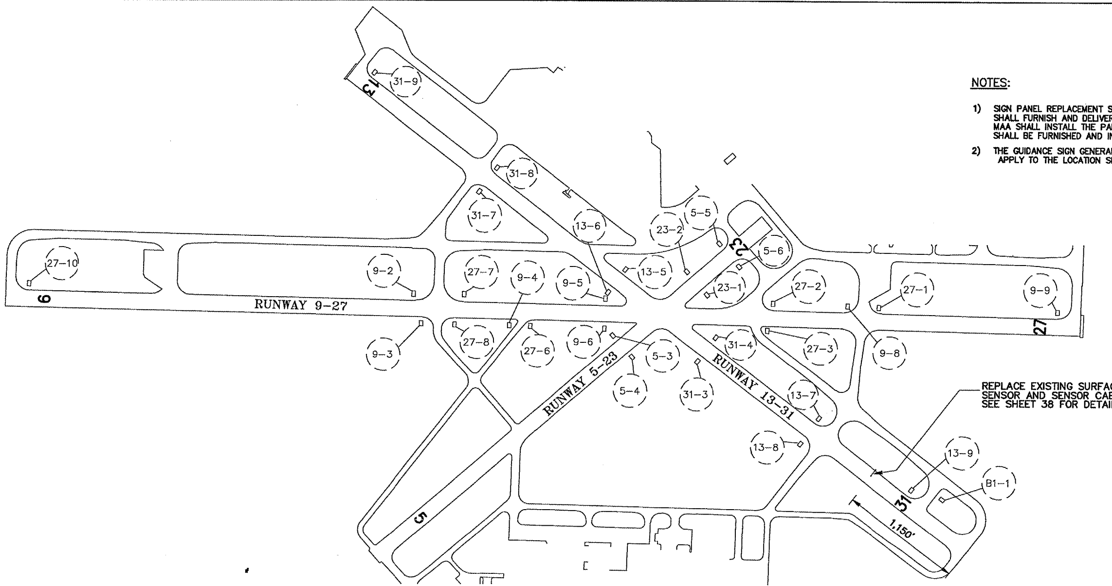
SUPPLY TAXIWAY GUIDANCE SIGN PANELS SIZE 3, STYLE 2, CLASS 2
