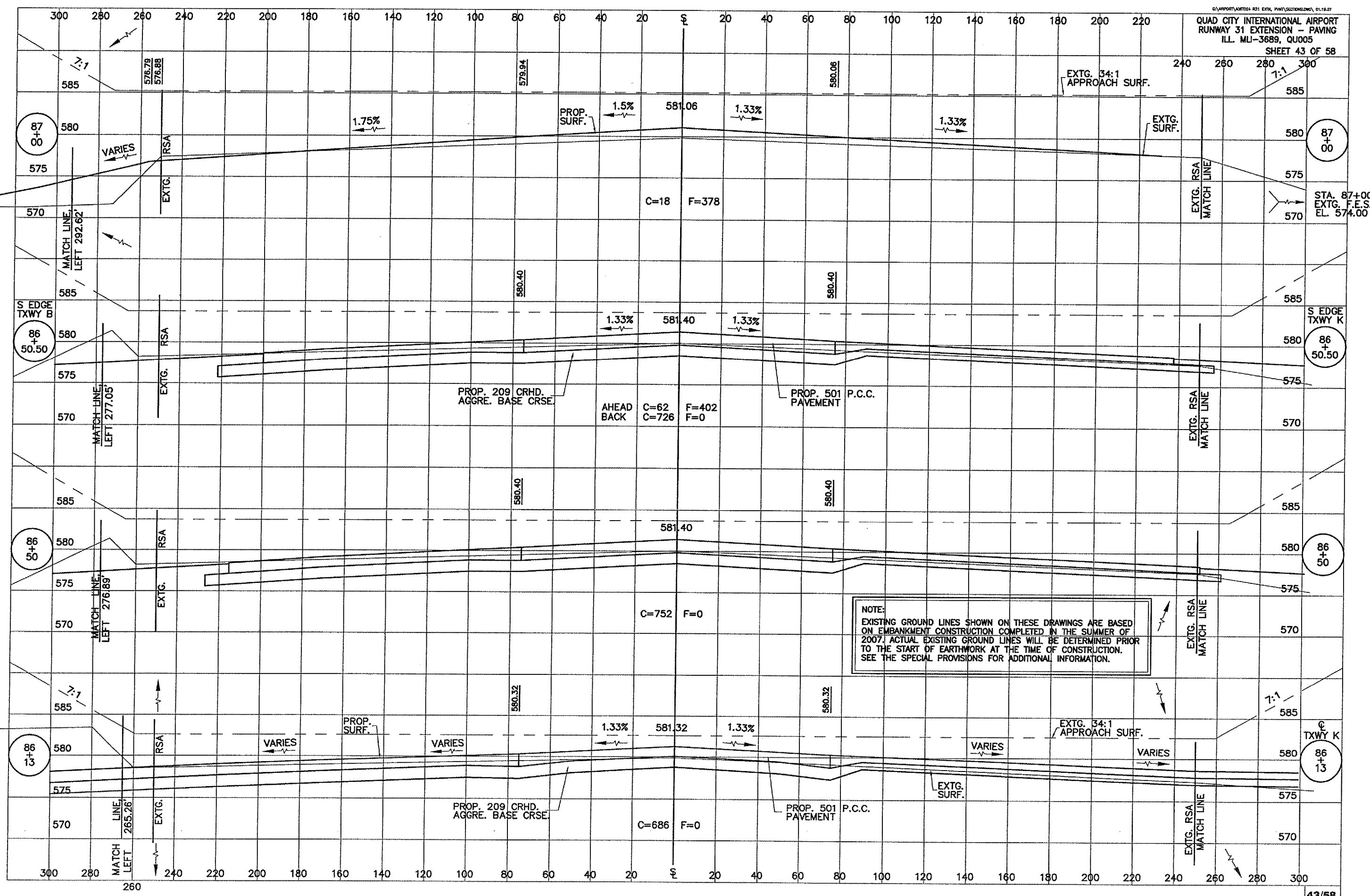
RUNWAY 31 CROSS SECTIONS, STA 86+13 TO STA 87+00
