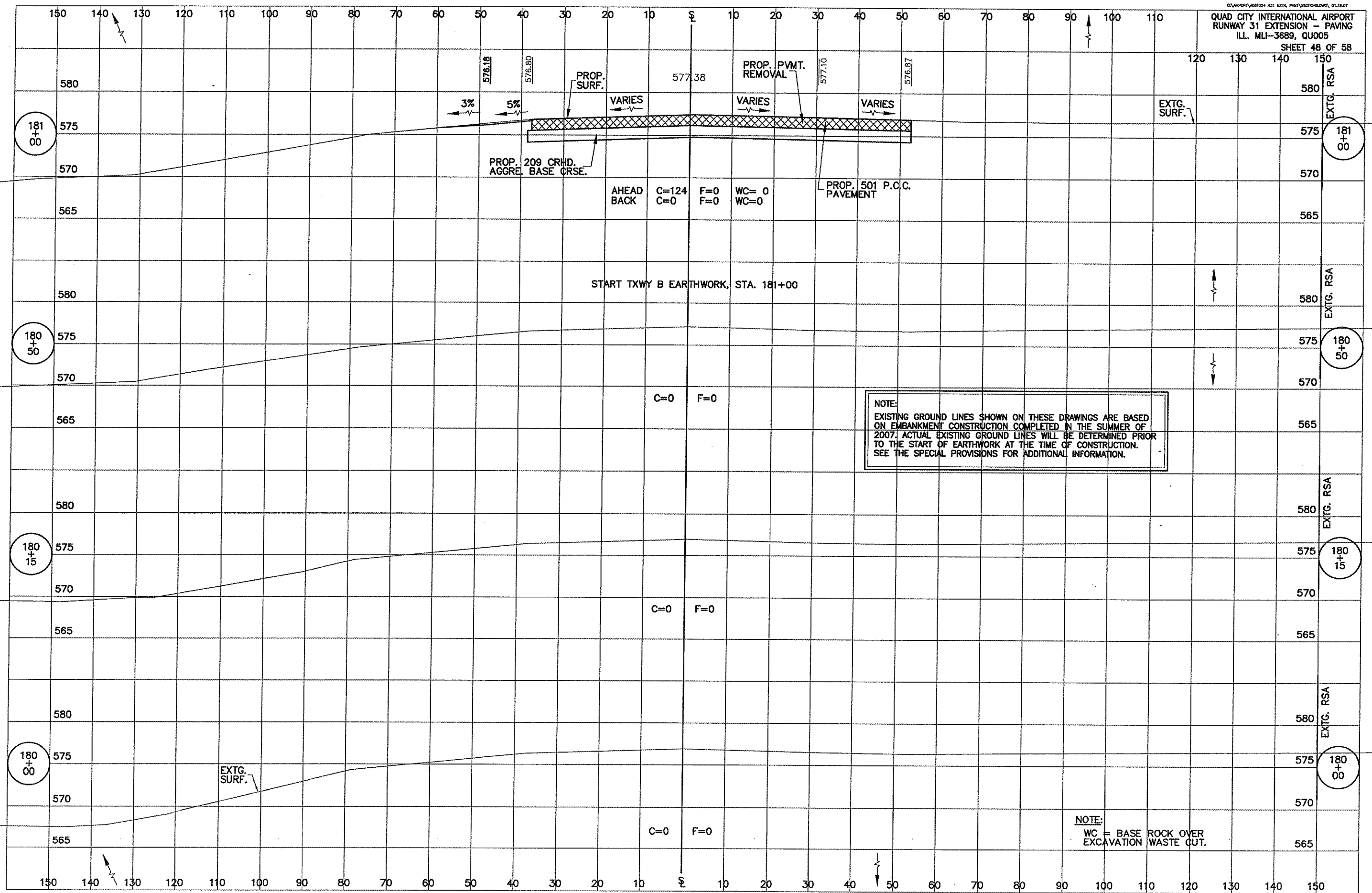
TAXIWAY B CROSS SECTIONS, STA 180+00 TO STA 181+00
