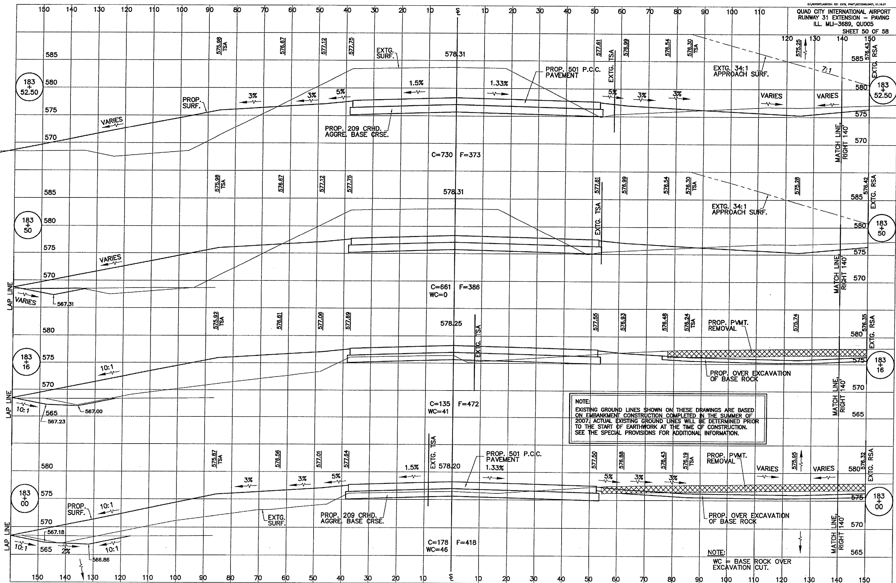
TAXIWAY B CROSS SECTIONS, STA 183+00 TO STA 183+52.50
