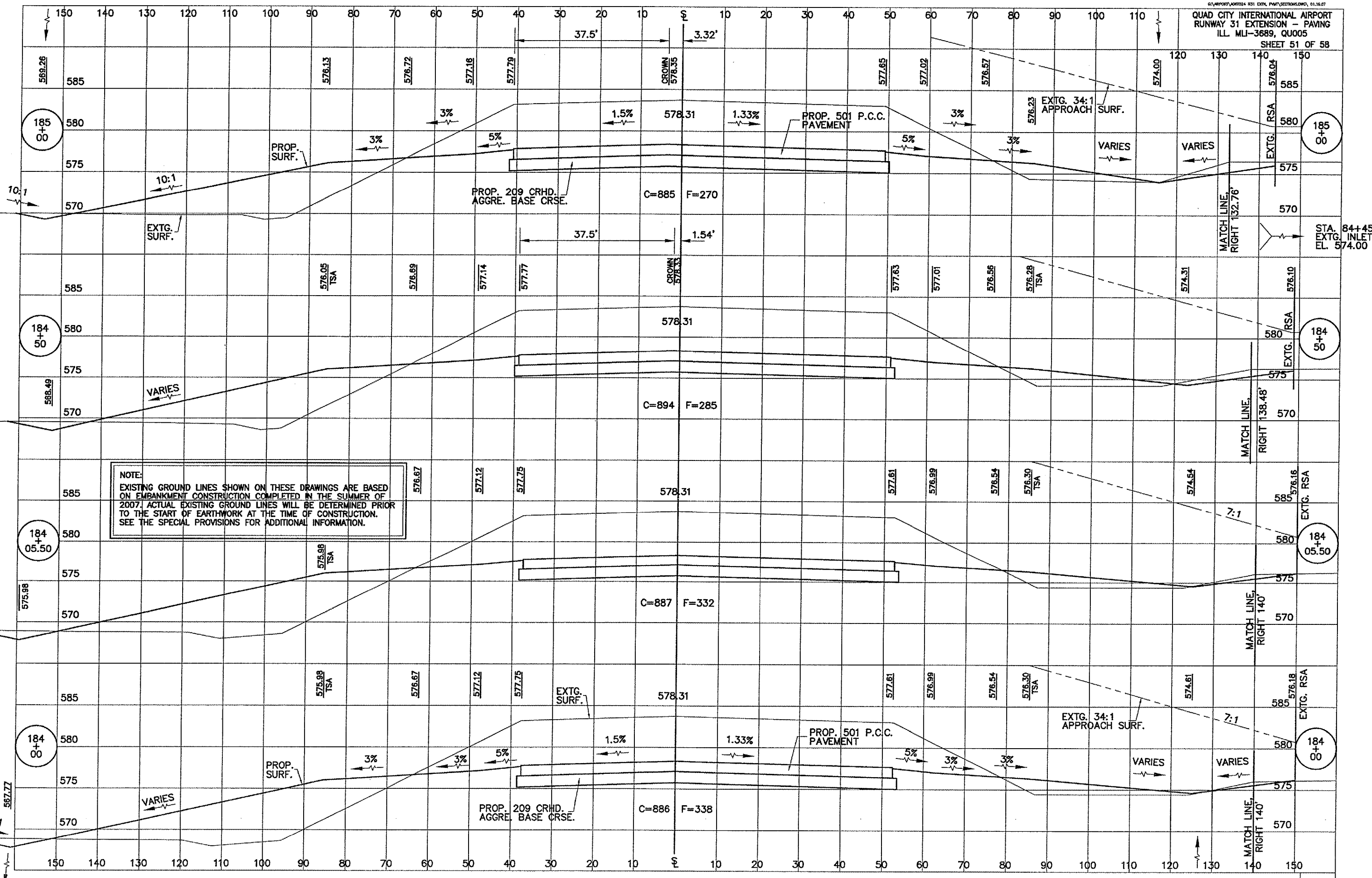
TAXIWAY B CROSS SECTIONS, STA 184+00 TO STA 185+00
