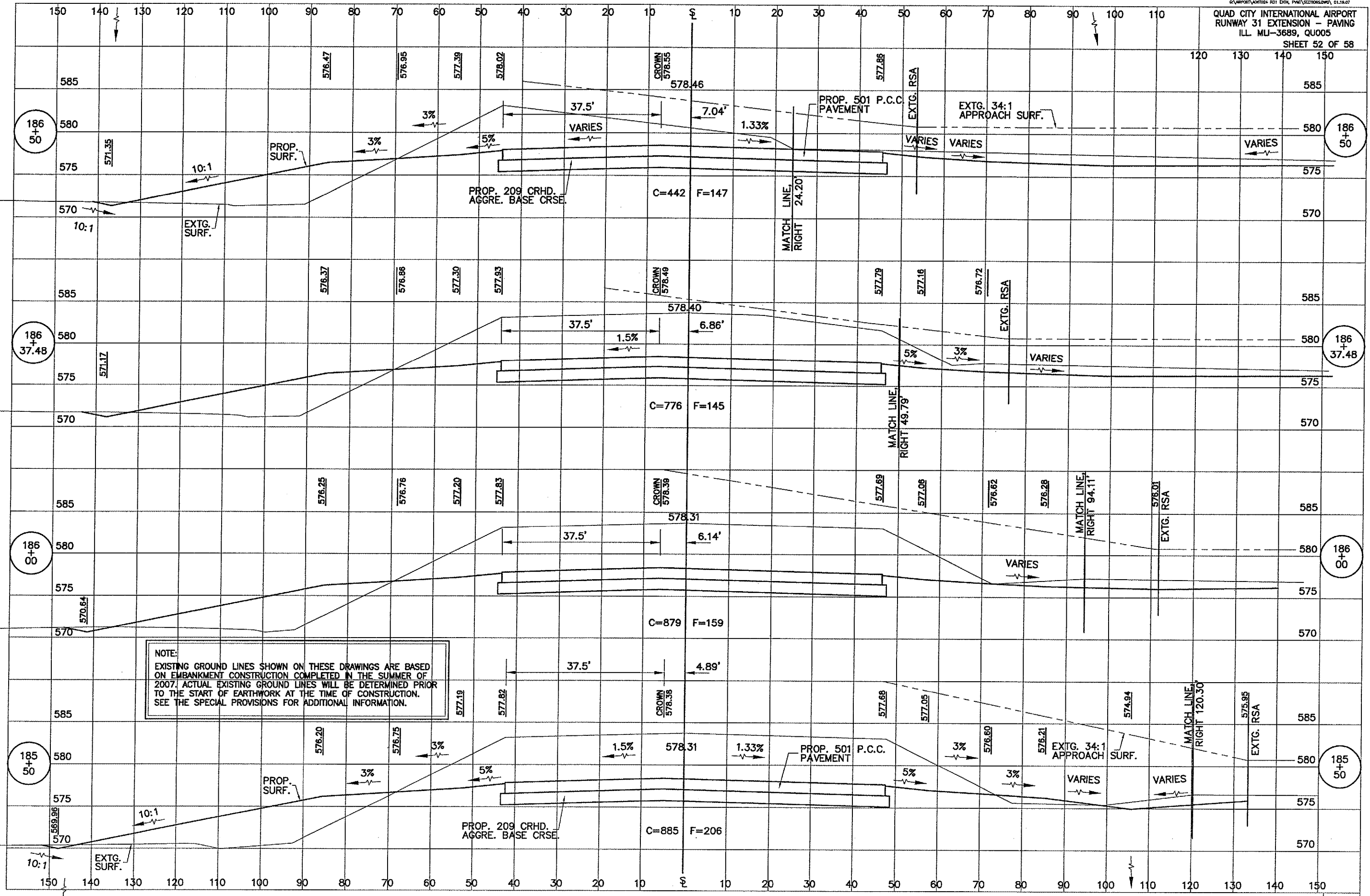
TAXIWAY B CROSS SECTIONS, STA 185+50 TO STA 186+50
