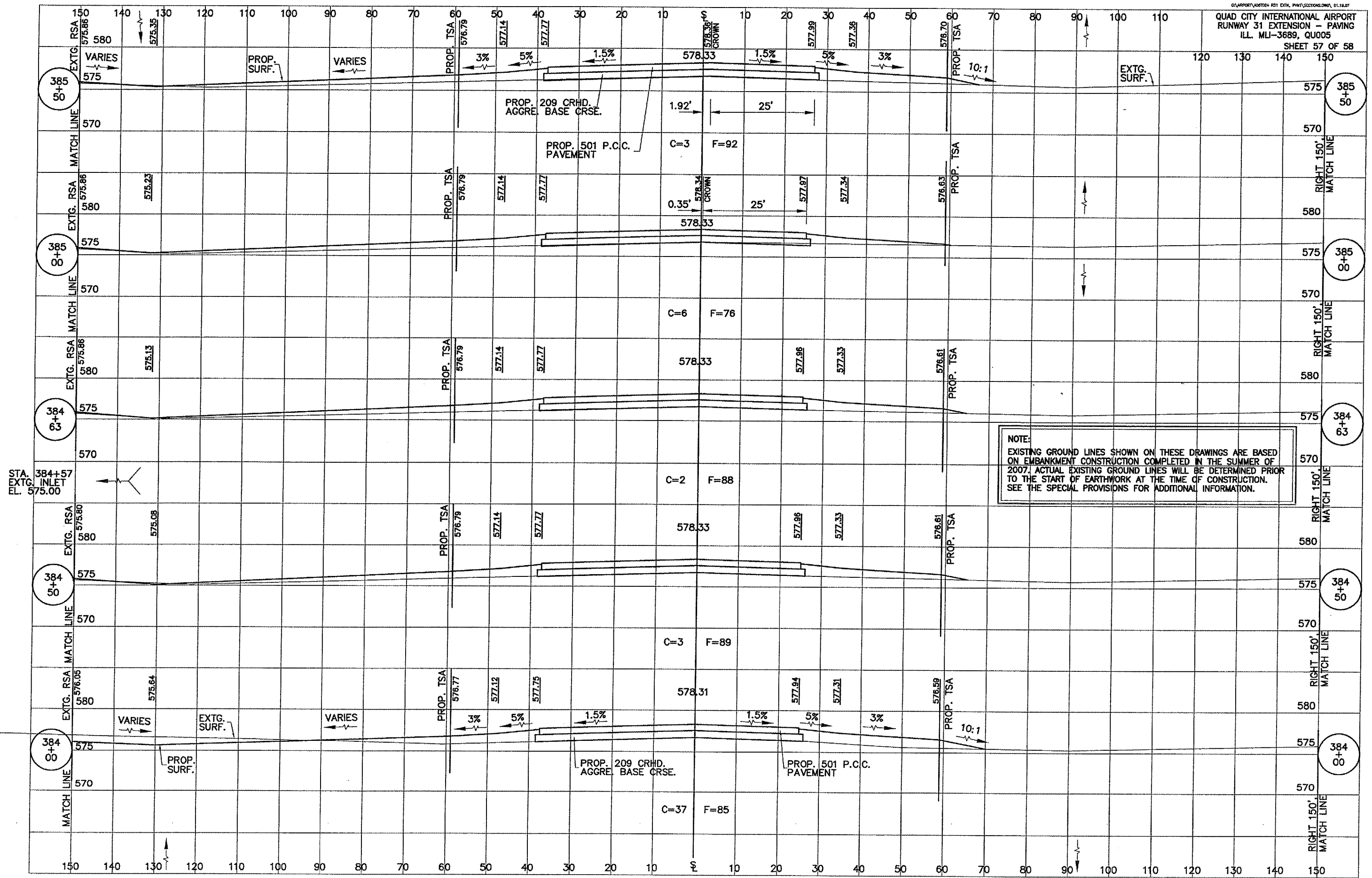
TAXIWAY K CROSS SECTIONS, STA 384+00 TO STA 385+50
