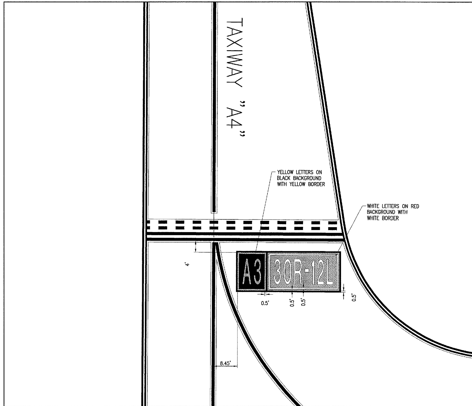
DETAIL "A" 1"=10'
