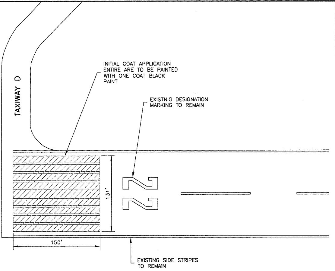
EXISTING THRESHOLD REMOVAL RUNWAY 22
