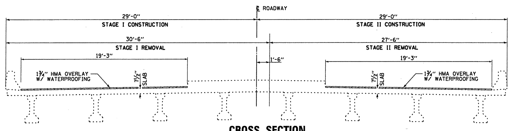
CROSS SECTION SPANS 1 AND 4 LOOKING EAST
