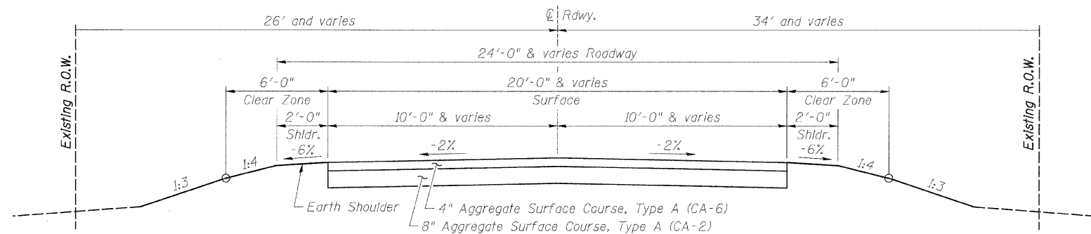
PROPOSED ROADWAY TYPICAL SECTION STA. 18+75 - STA. 21+25 (Looking North)
