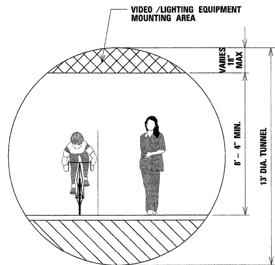
TYPICAL TUNNEL SECTION NOT TO SCALE
