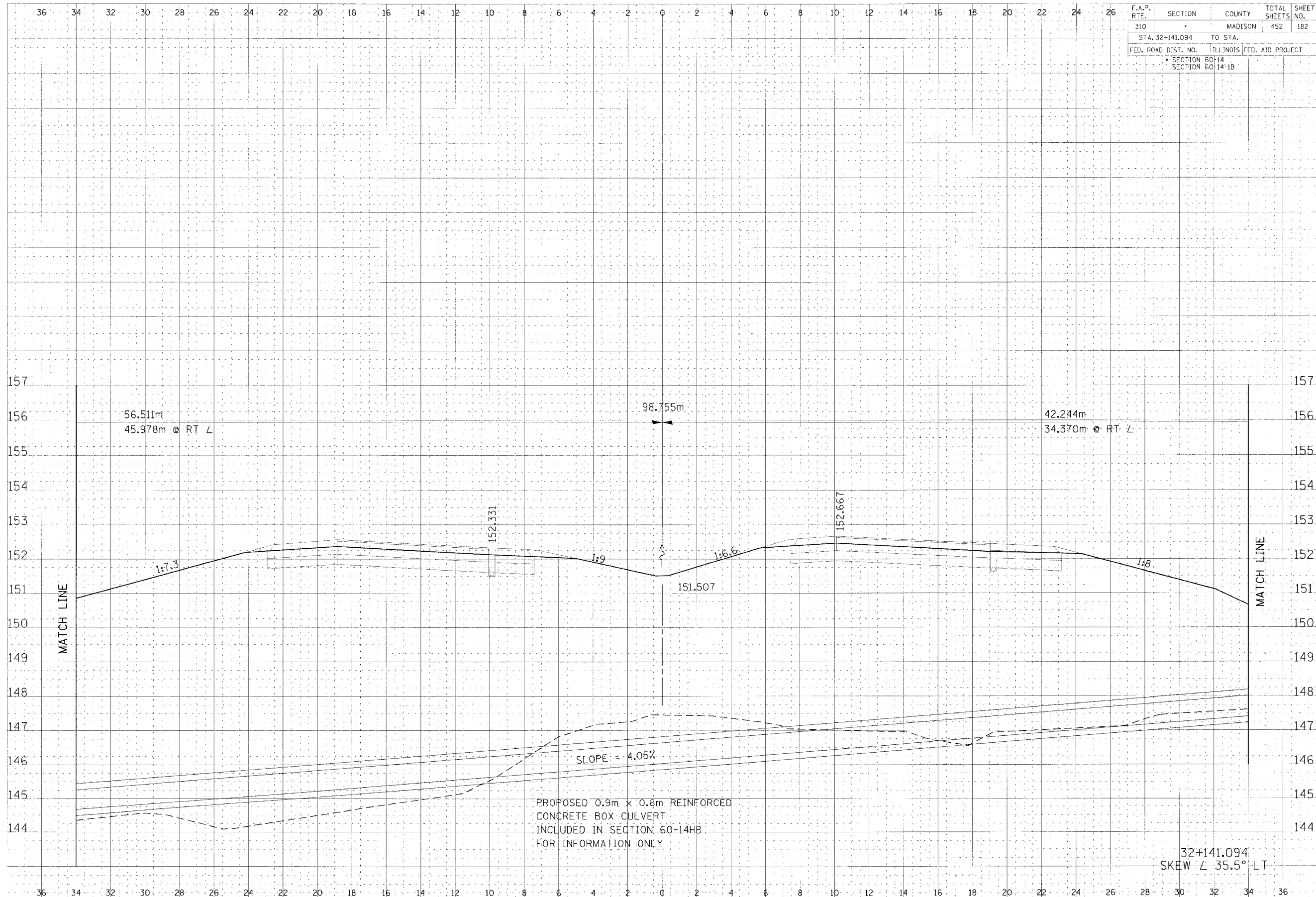
CULVERT PROFILE, FAP ROUTE 310, STA 32+141.094
