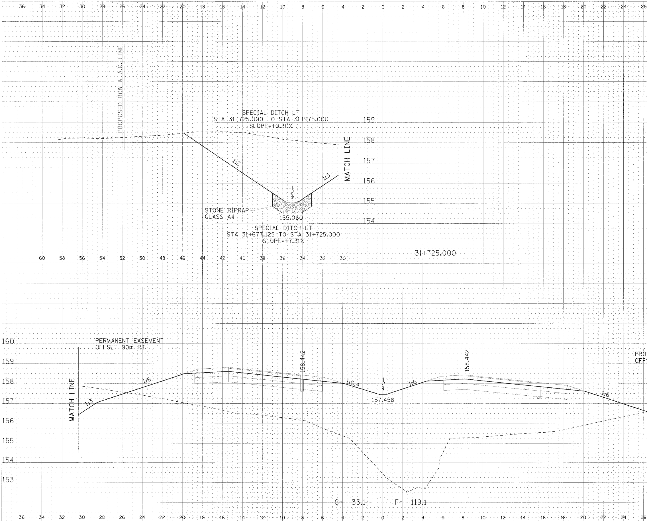
CROSS SECTION, FAP ROUTE 310, STA 31+725.000
