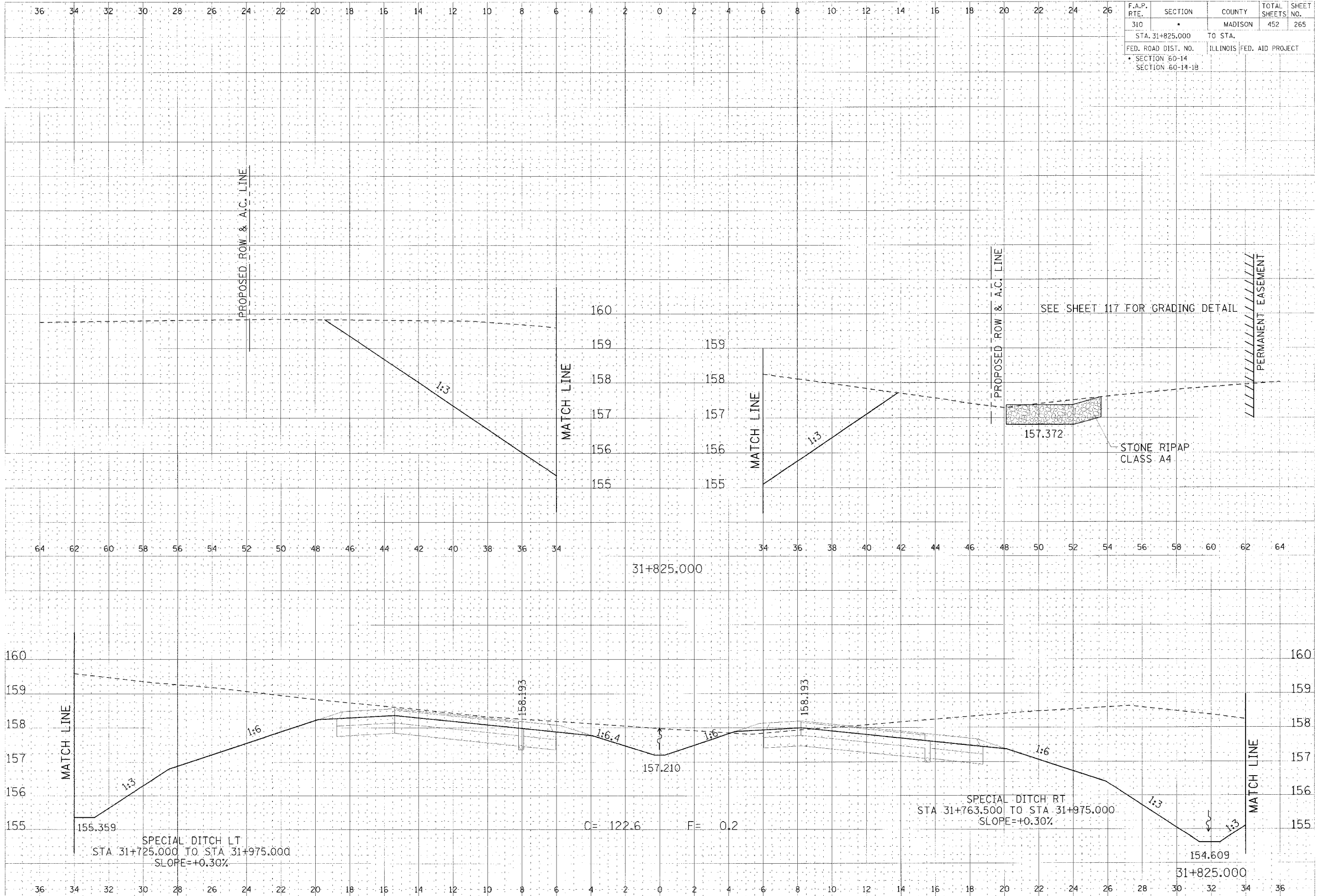
CROSS SECTION, FAP ROUTE 310, STA 31+825.000
