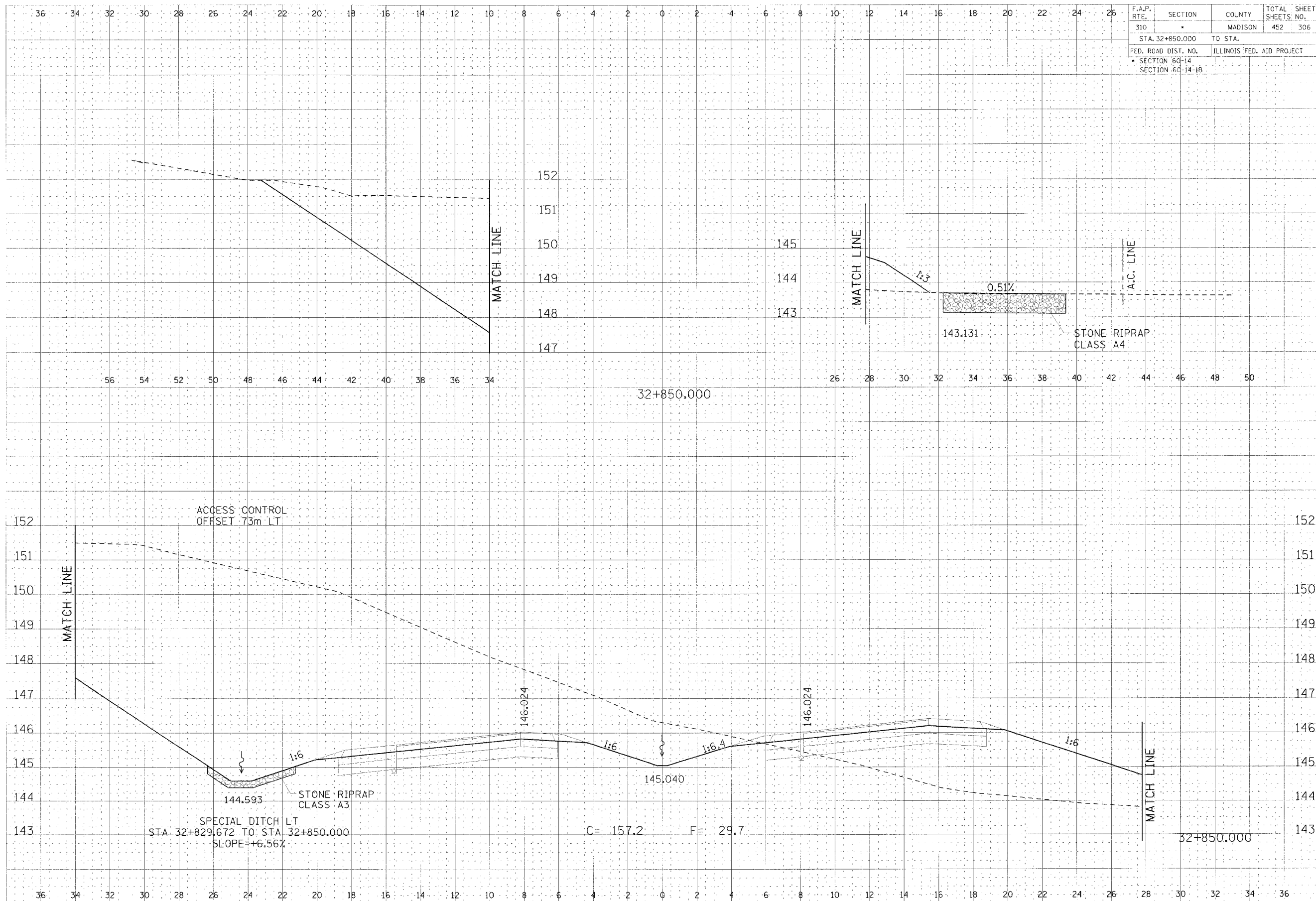
CROSS SECTION, FAP ROUTE 310, STA 32+850.000
