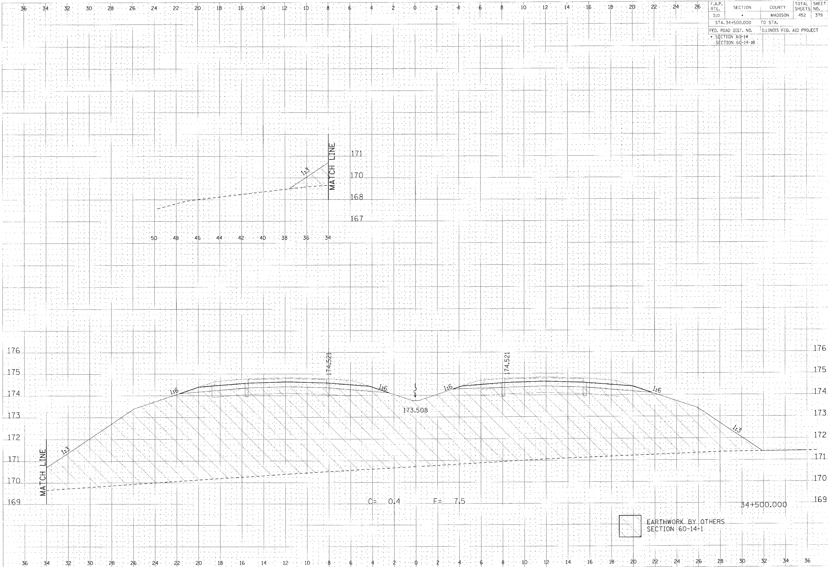
CROSS SECTION, FAP ROUTE 310, STA 34+500.000
