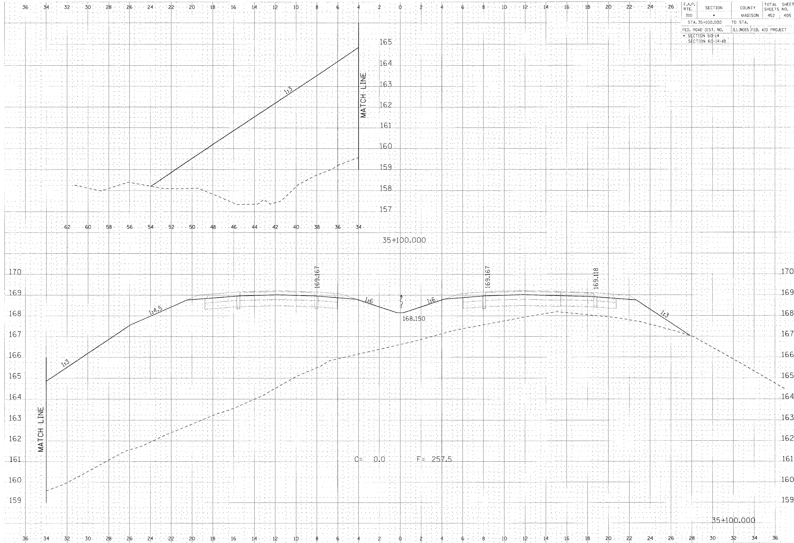
CROSS SECTION, FAP ROUTE 310, STA 35+100.000
