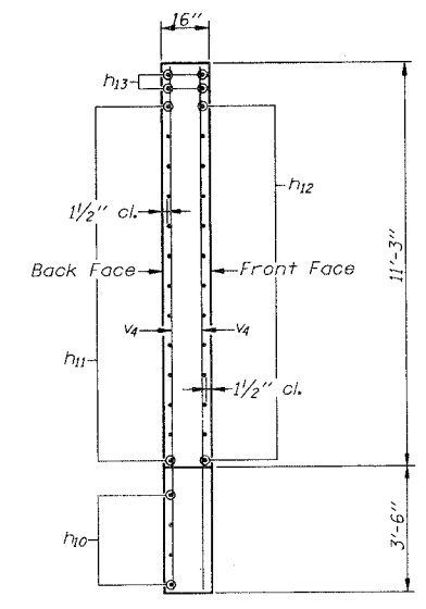
SEC. F-F
