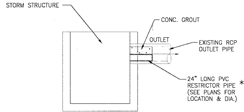
RESTRICTOR DETAIL
