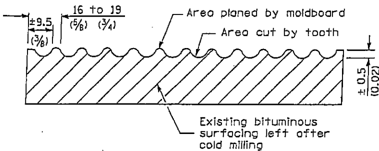
SECTION B-B PROJECTED PERPENDICULAR TO CENTERLINE
