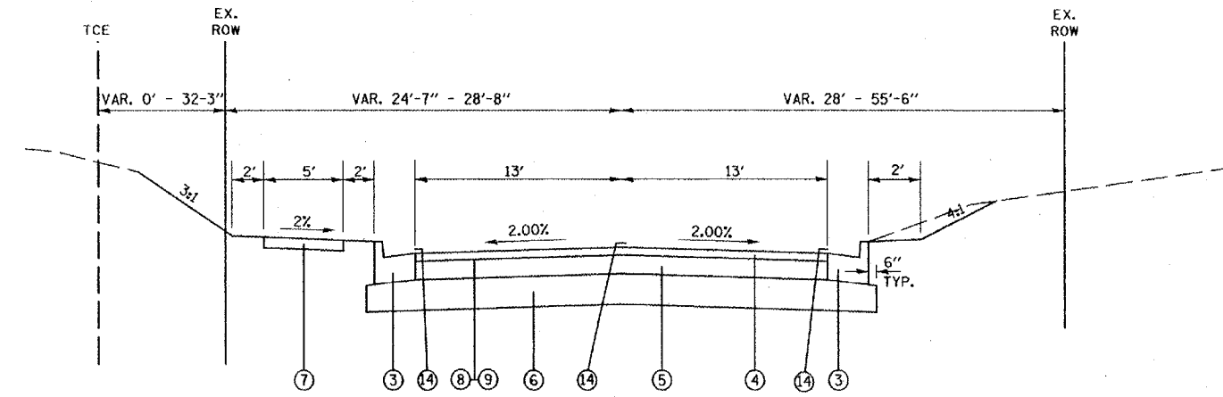
PROPOSED TYPICAL SECTION SEIBERT ROAD STA. 16+80.00 TO STA. 17+35.00
