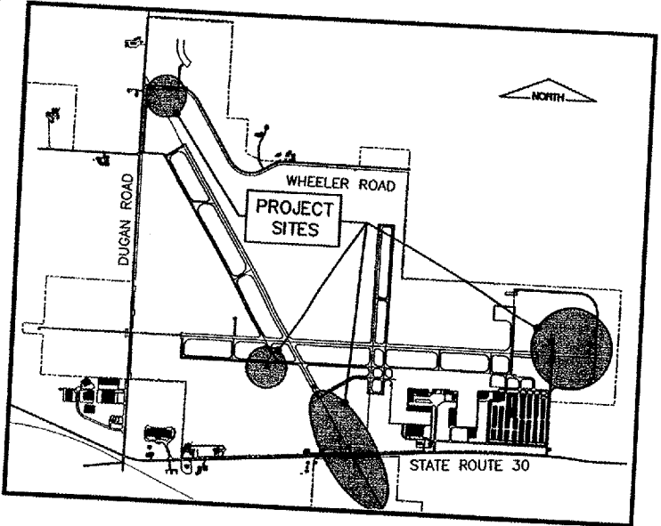
SITE PLAN
