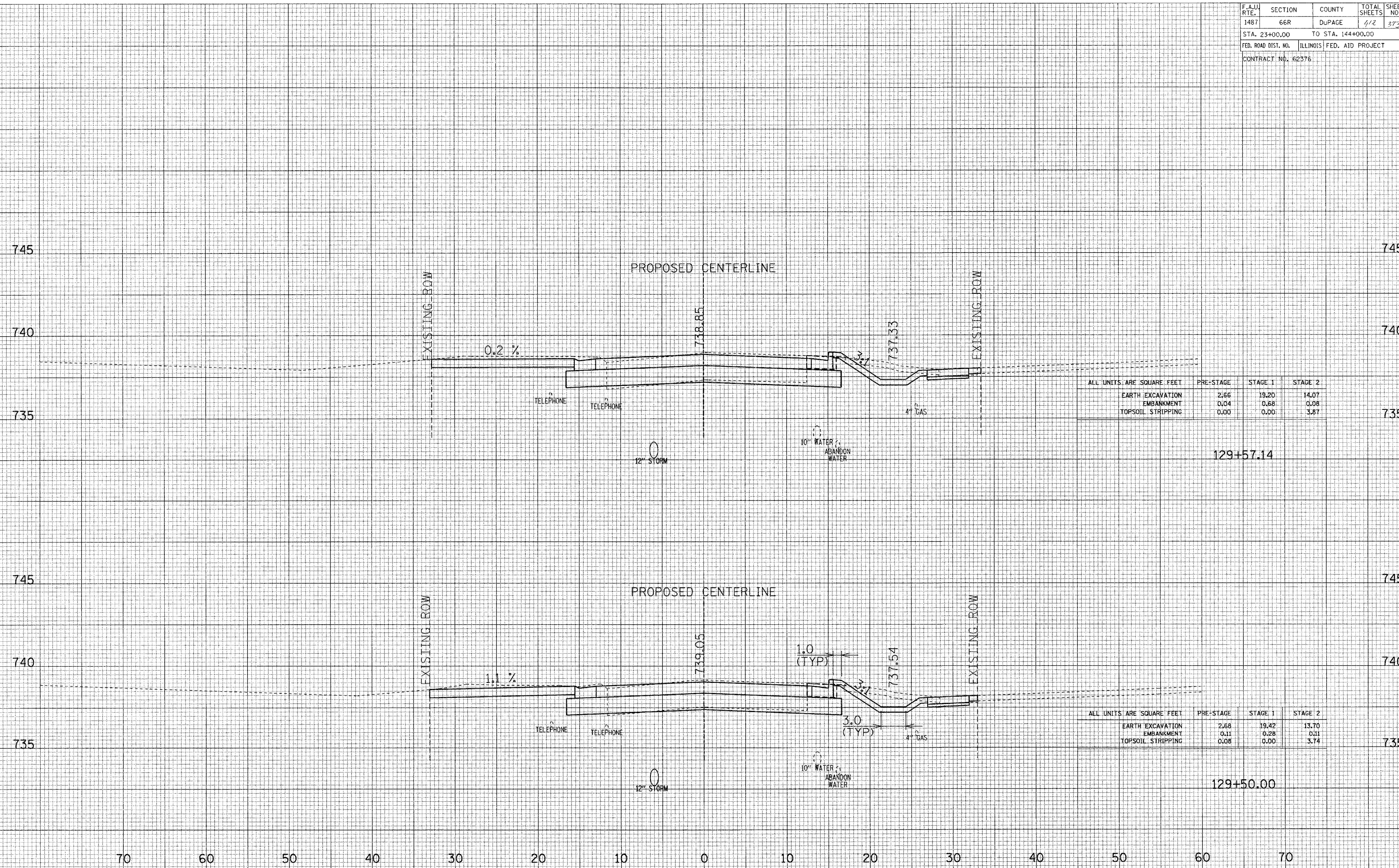
MAPLE AVENUE CROSS SECTIONS
