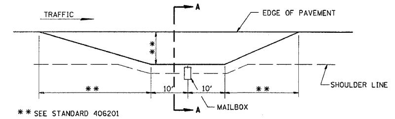
PLAN AT PRIVATE & COMMERCIAL ENTRANCES (DO NOT RESURFACE FIELD ENTRANCES)
