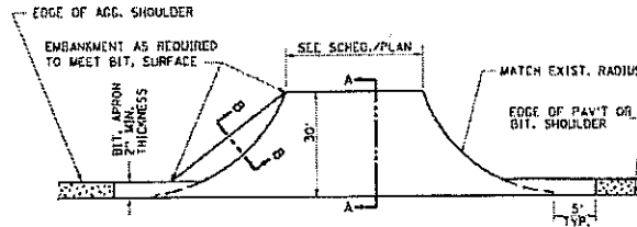
PLAN AT SIDE ROADS
