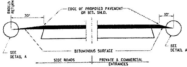
SECTION A-A DETAILS AT ENTRANCES & SIDE ROADS
